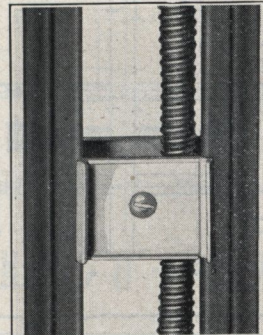
Through-bolted Clip
