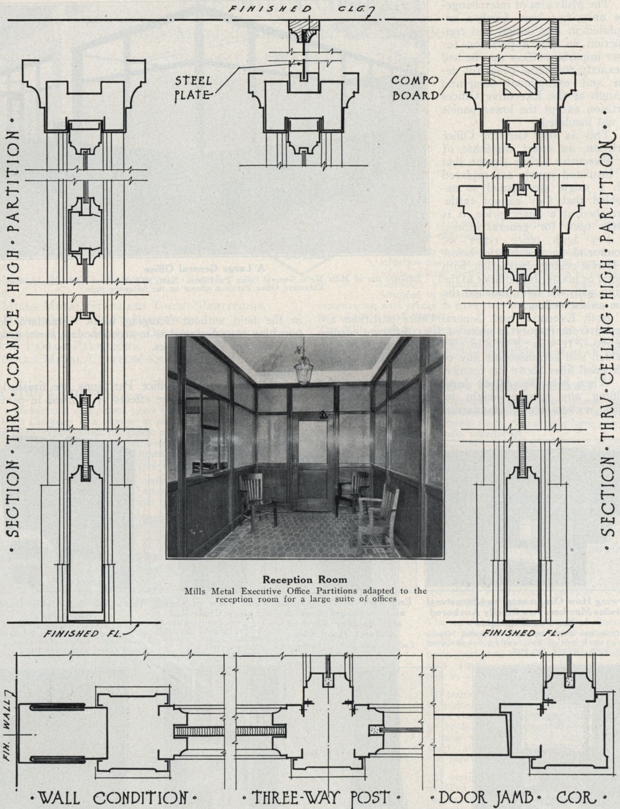
• DETAILS • OF • EXECUTIVE • OFFICE • PARTITIONS • SCALE 3" = 1'-0"
